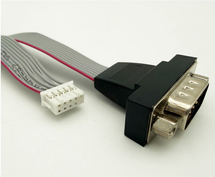
COM-connector f. RS232-Header (2.00mm Pitch)
